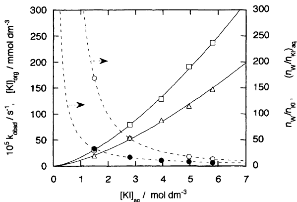
Fig. 2. The influences of [KI]_{aq} on [KI]_{org} , k_{obsd} , and n_W/n_{KI} for the reaction between 1-bromodecane and aqueous KI using cyclohexanol as an organic solvent. (Δ), k_{obsd} ; (□), [KI]_{org} ; (○), n_W/n_{KI} ; (●), (n_W/n_{KI})_{aq} , the molar ratio of water to KI in the bulk aqueous phase.
