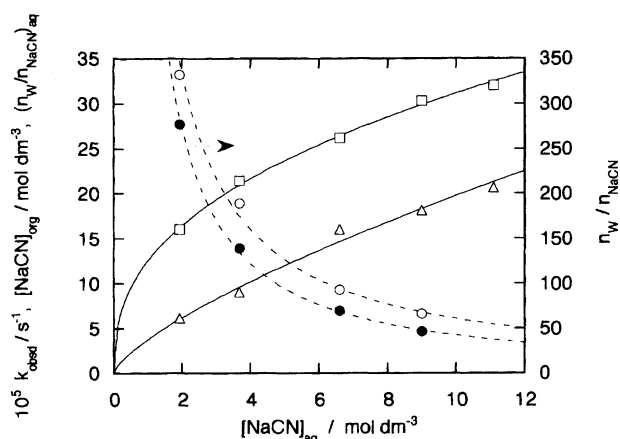
Fig. 3. The influences of [NaCN]_{aq} on [NaCN]_{org} , k_{obsd} , and n_W/n_{NaCN} for the reaction between 1-bromodecane and aqueous NaCN using cyclohexanol as an organic solvent. (Δ), k_{obsd} ; (□), [NaCN]_{org} ; (○), n_W/n_{NaCN} ; (●), (n_W/n_{NaCN})_{aq} , the molar ratio of water to NaCN in the bulk aqueous phase.
