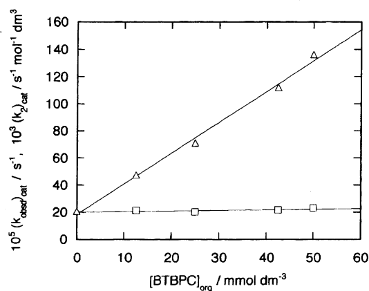
Fig. 5. The dependence of the rate of the BTBPC-catalyzed reaction between 1-bromodecane and aqueous sodium cyanide on the BTBPC concentration in cyclohexanol. ( \Delta ), k_{\text{obsd}} ; ( \square ), (k_2)_{\text{cat}} .
