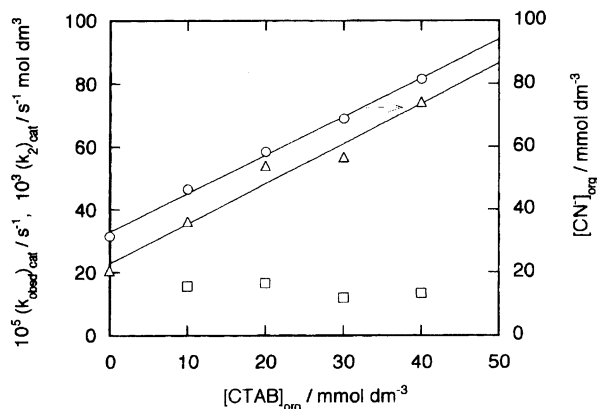
Fig. 4. The dependence of the rate of the CTAB-catalyzed reaction between 1-bromodecane and aqueous sodium cyanide on the CTAB concentration in cyclohexanol. ( \Delta ), k_{\text{obsd}} ; ( \square ), (k_2)_{\text{cat}} ; ( \circ ), [\text{CN}^-]_{\text{org}} .
